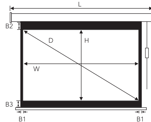
Installation Diagram:
