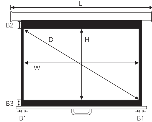
Installation Diagram:
