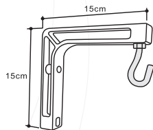
"L" Screen Bracket 15cm
