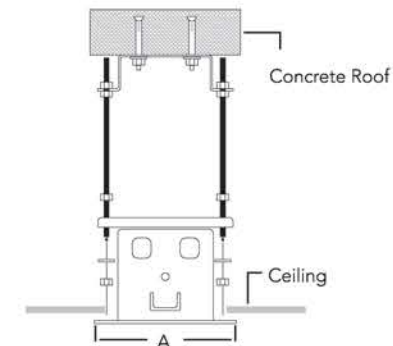
Installation Diagram
