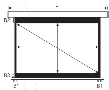
Installation Diagram
