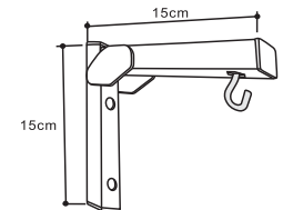
Foldable Screen Bracket
