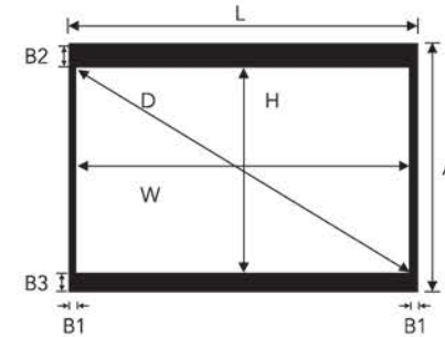
Installation Diagram:
