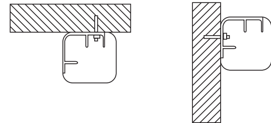
Installation Diagram:
