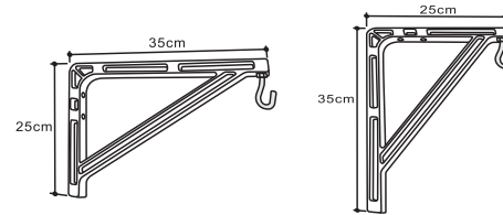
"L" Screen Bracket 35 or 25cm
